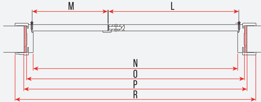
RESİM/PICTURE 3: SALON KAPISI GENEL KESİT DOUBLE WING DOOR'S GENERAL CROSS SECTION
