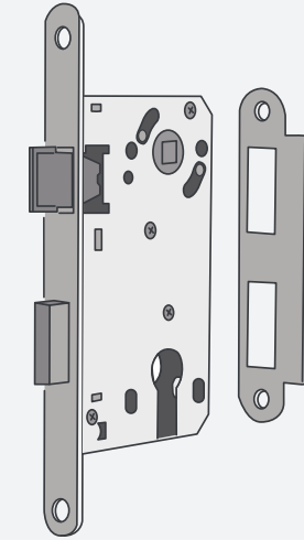
SESSİZ BARELLİ KİLİT SILENT BARELLI LOCK
