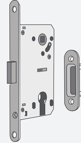
SESSİZ MANYETİK BARELLİ KİLİT SILENT MAGNETIC BARELLI LOCK
